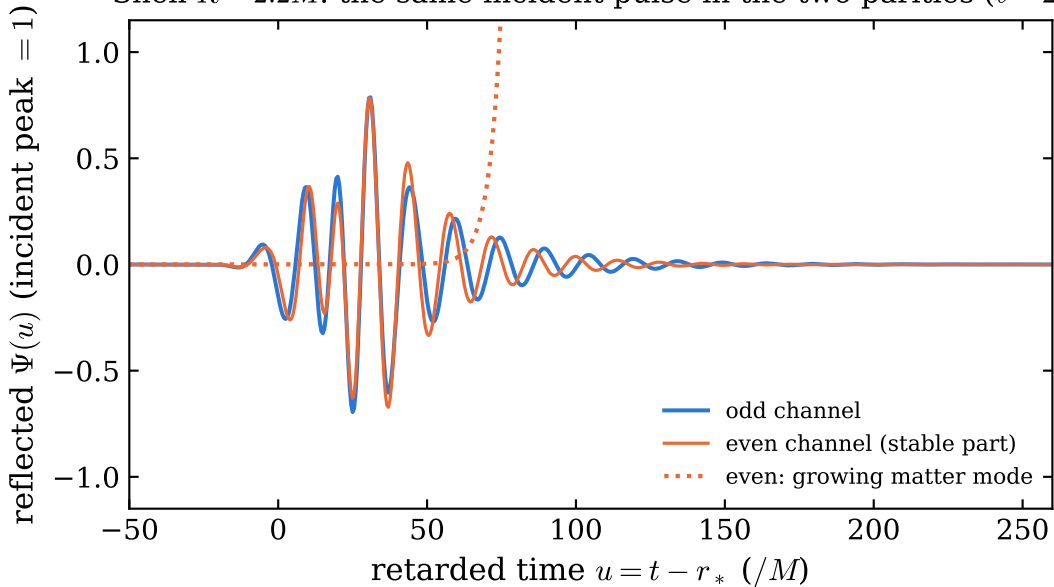
Shell R = 2.2M : the same incident pulse in the two parities ( \ell = 2 )
